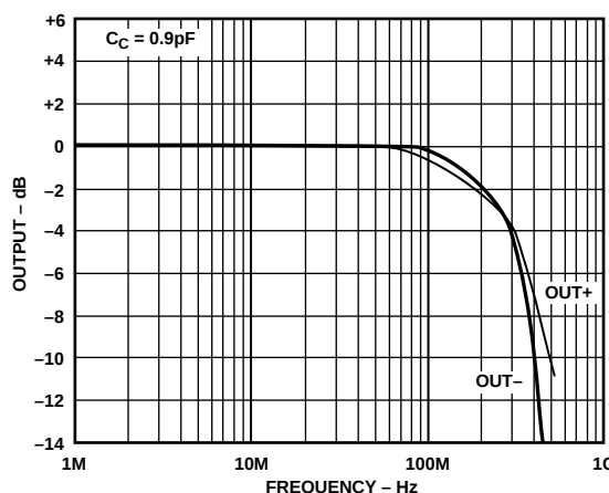
Figure 48. Differential Driver Frequency Response
